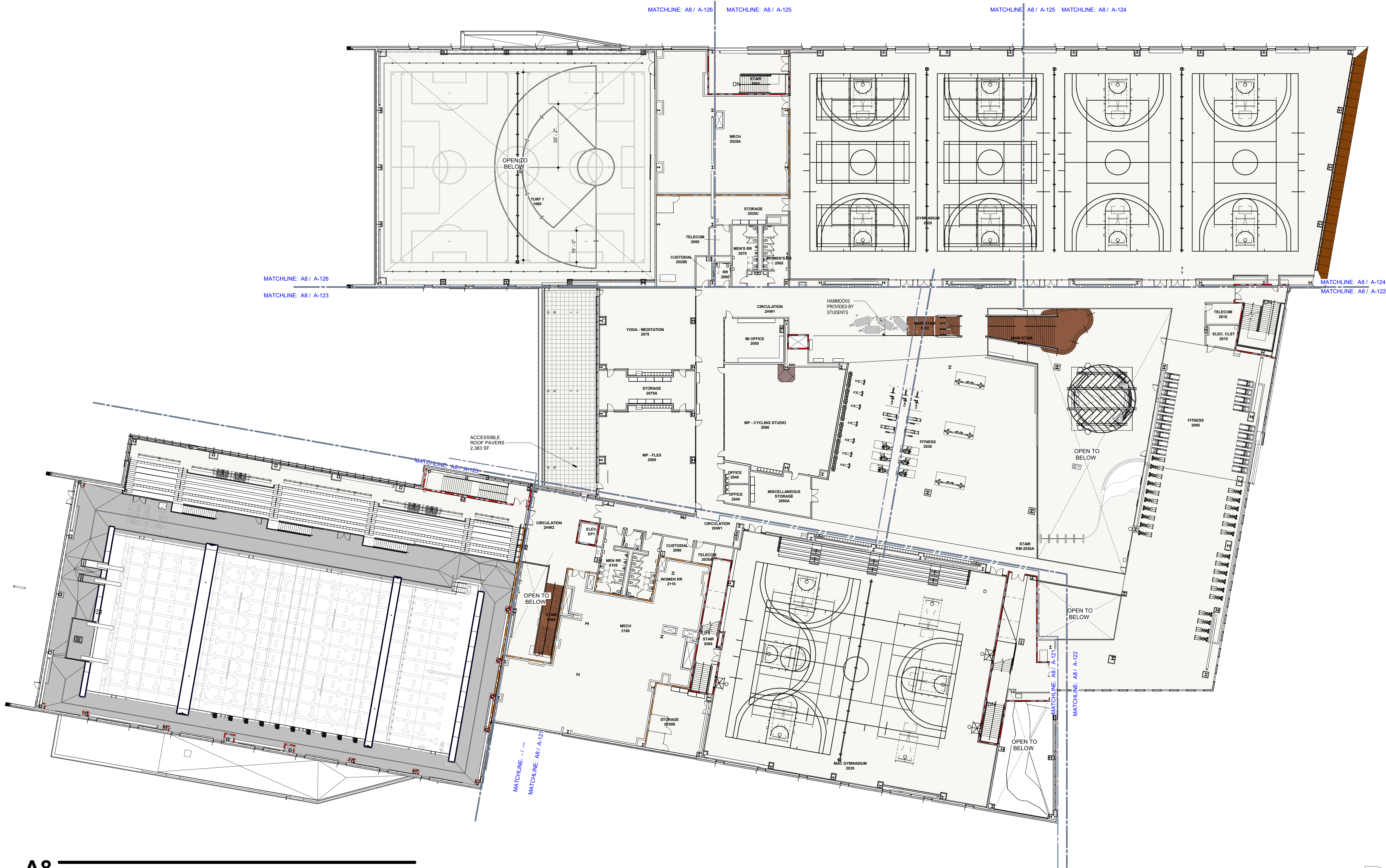
A8 OVERALL FURNITURE PLAN - LEVEL 02 A-1002 SCALE: 1" = 20'-0"
