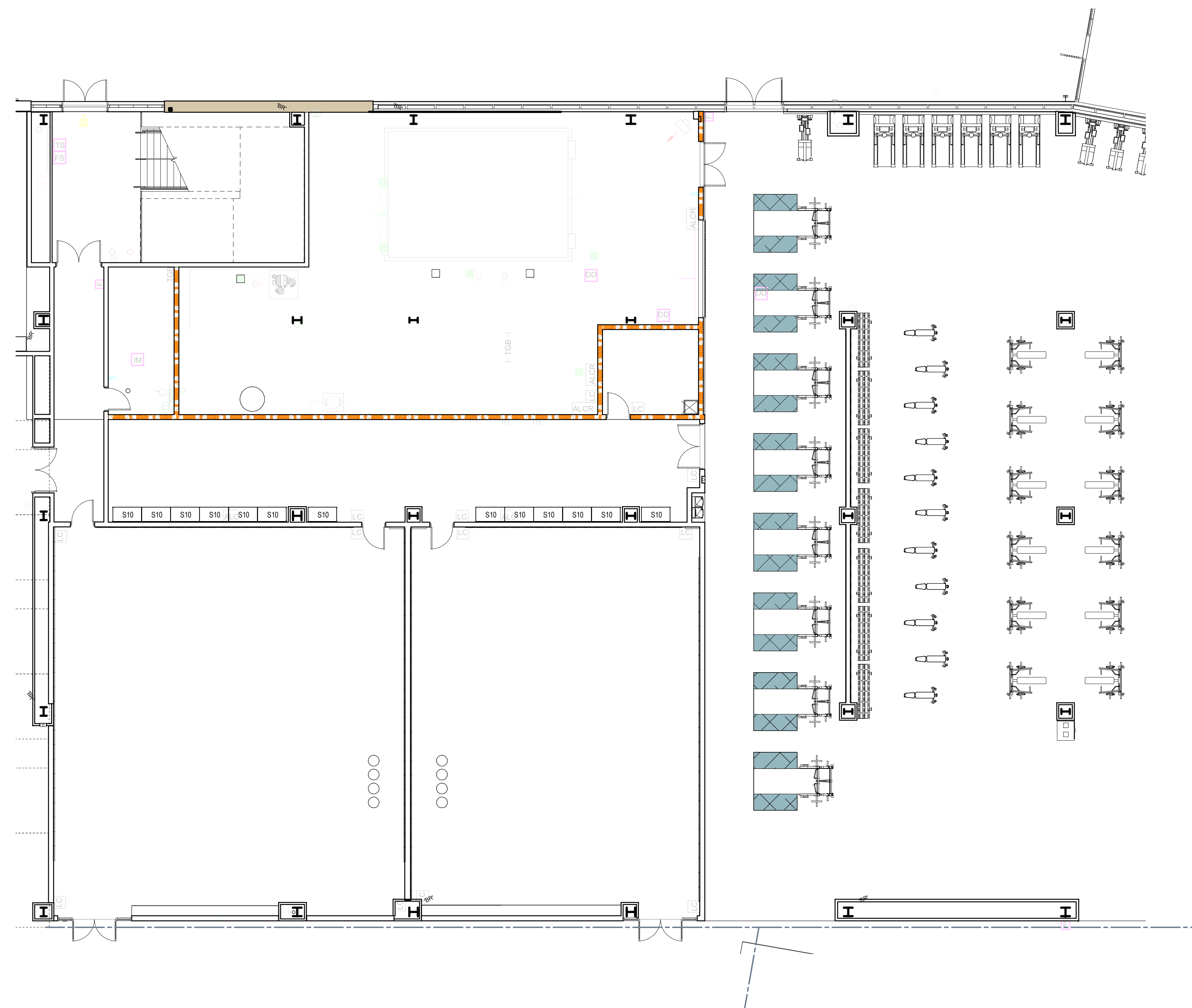
1 FURNITURE PLAN - LEVEL 01 - AREA 5 A-1008 SCALE: 1/8" = 1'-0"
